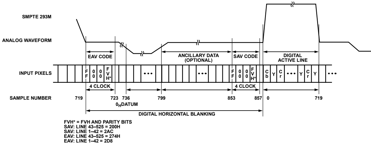
Figure 135. EAV/SAV Input Data Timing Diagram (SMPT 293M)
