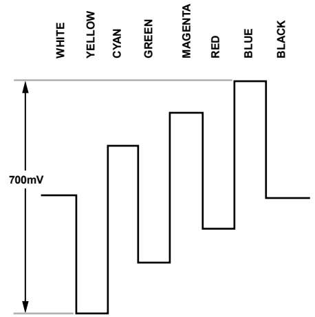
Figure 119. Pb Levels—PAL
