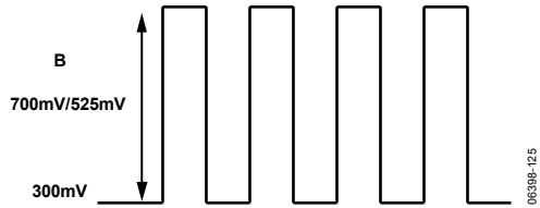
Figure 124. SD/ED RGB Output Levels—RGB Sync Disabled
