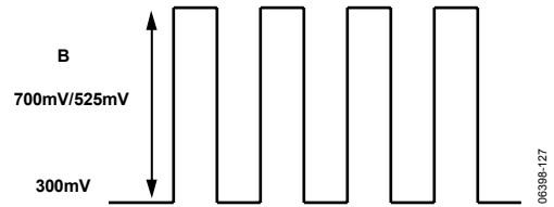
Figure 126. HD RGB Output Levels—RGB Sync Disabled
