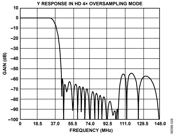
Figure 28. HD 4x Oversampling, Y Filter Response
