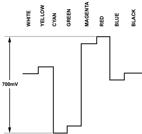
Figure 115. Pr Levels—NTSC
