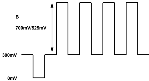
Figure 125. SD/ED RGB Output Levels—RGB Sync Enabled
