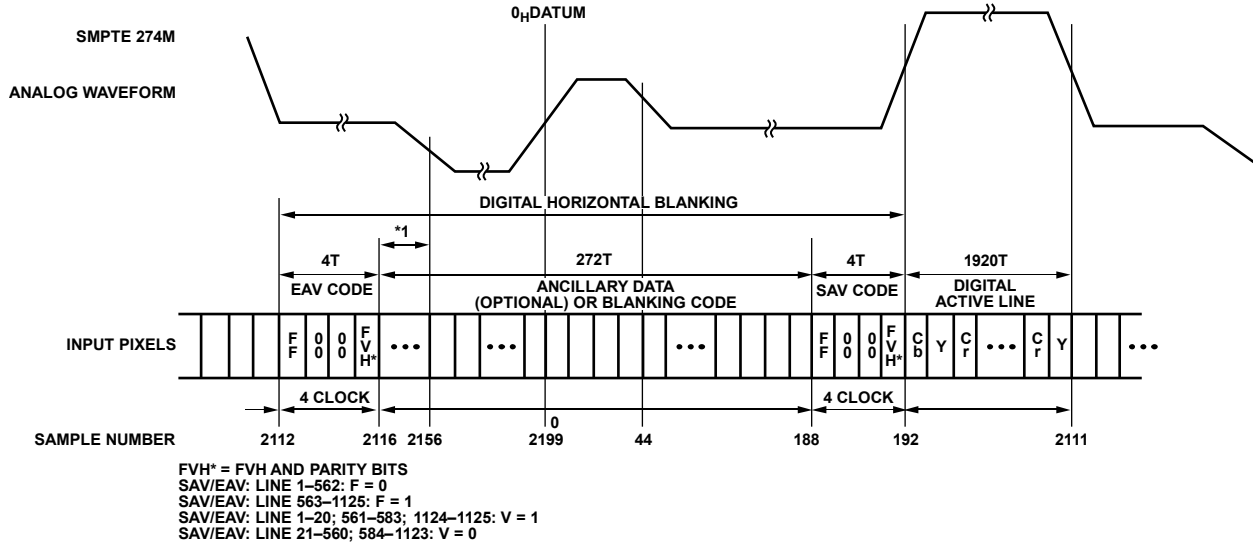
Figure 134. EAV/SAV Input Data Timing Diagram (SMPT 274M)
