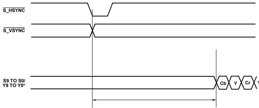
Figure 18. SD Input Timing Diagram (Timing Mode 1)
