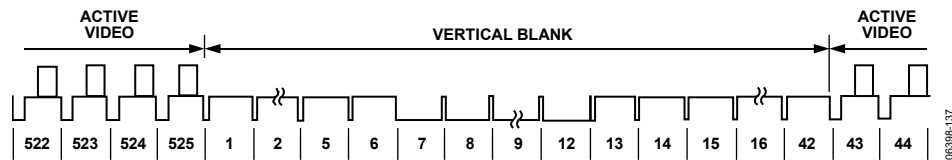
Figure 136. SMPT 293M (525p)
