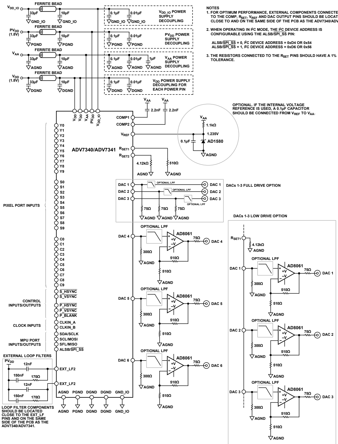
Figure 90. ADV7340/ADV7341 Typical Application Circuit
