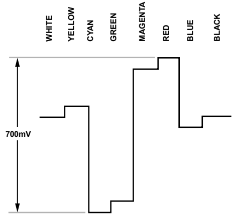
Figure 118. Pr Levels—PAL
