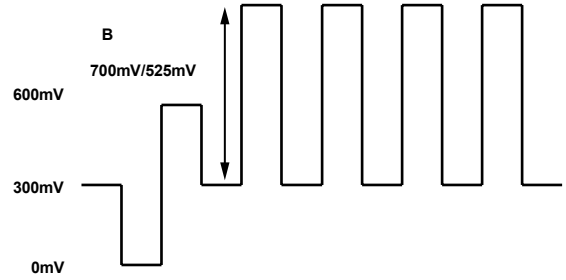
Figure 127. HD RGB Output Levels—RGB Sync Enabled
