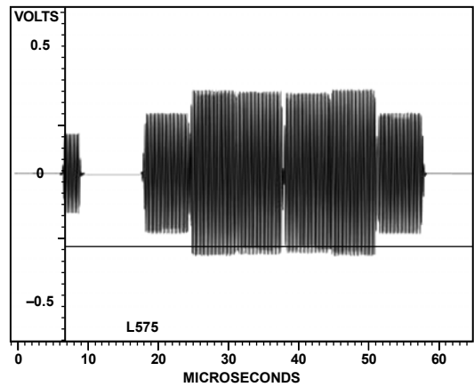
Figure 132. PAL Luma
