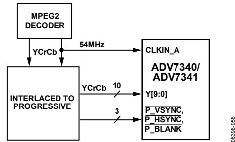
Figure 58. ED Only (at 54 MHz) Example Application
