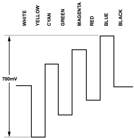
Figure 116. Pb Levels—NTSC
