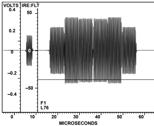
Figure 129. NTSC Luma
