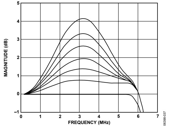
Figure 37. SD Luma SSAF Filter, Programmable Gain
